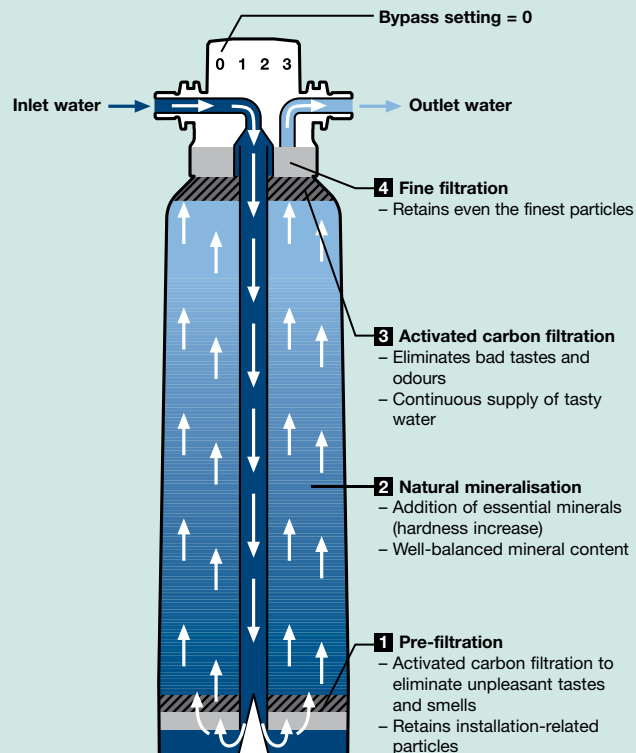
Structure of a bestmin filter cartridge
